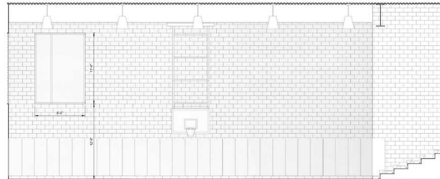
Gym Interior Elevation 2
