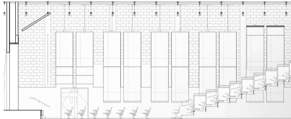
Auditorium Interior Elevation 1
